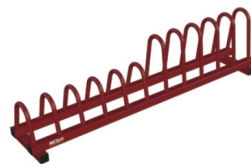
DF66 Weight Plate Holder Weight: 31kg LXWXH: 1700x300x440mm
