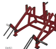
DH51 Squat High Pull Weight: 92kg LXWXH: 1767x1621x1042mm
